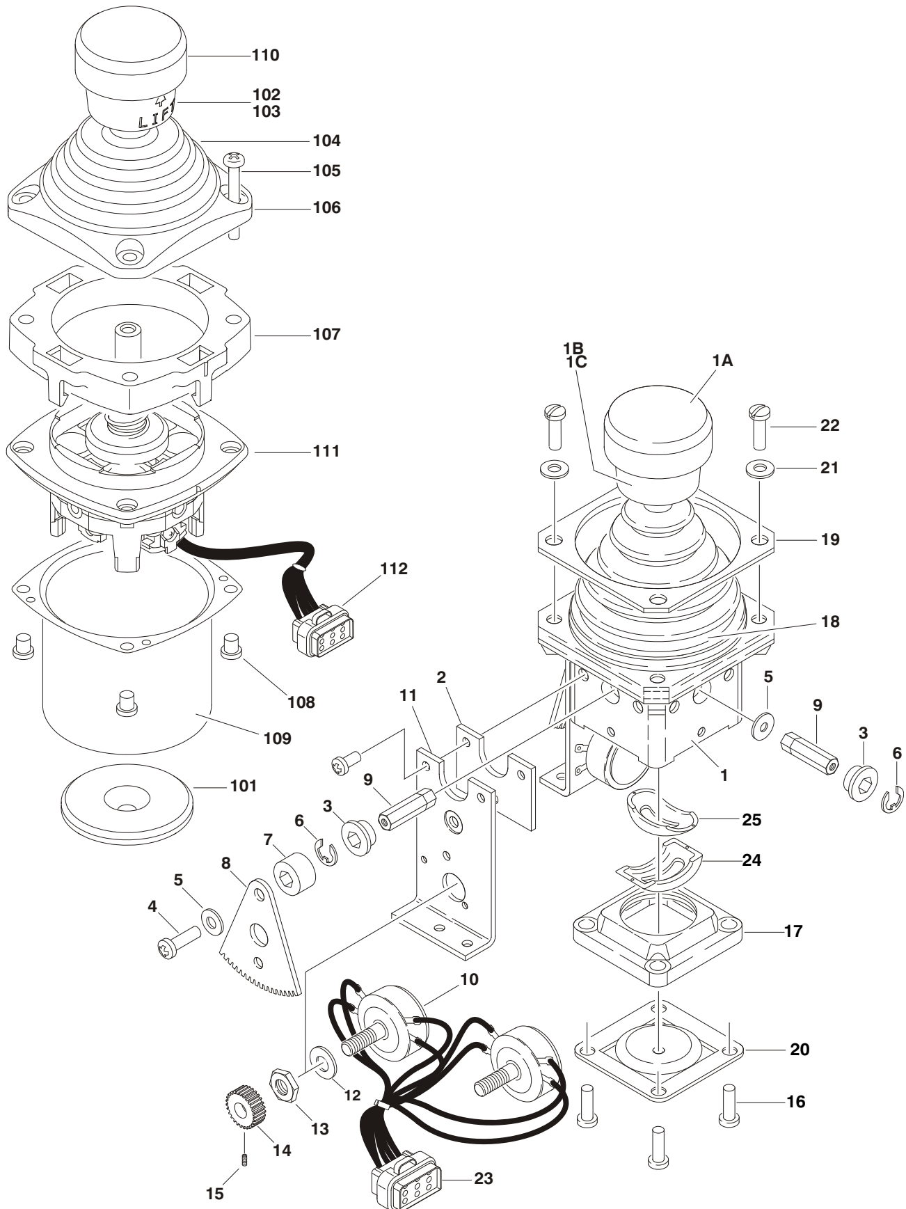
FIGURE 4-5. CONTROLLER ASSEMBLY (LIFT AND SWING)
