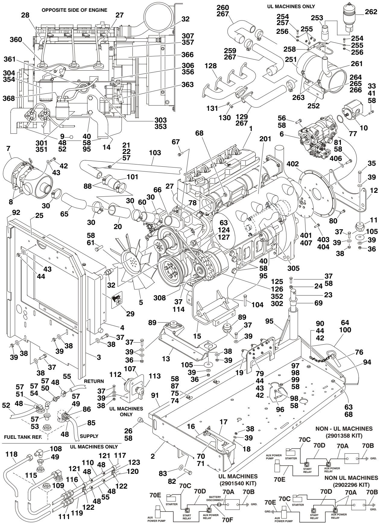
FIGURE 2-8. DEUTZ ENGINE INSTALLATION (S/N 0300069000 TO S/N 0300077490)
