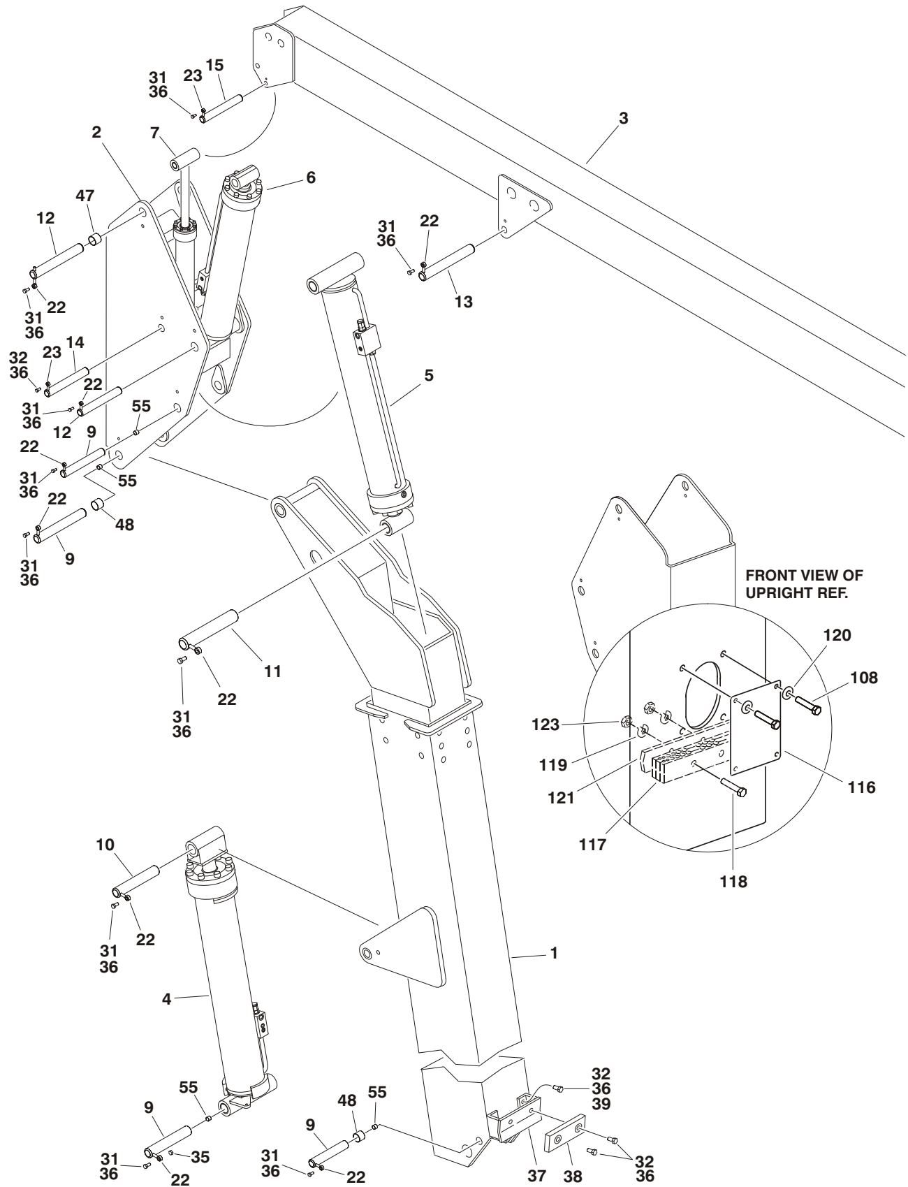
FIGURE 3-2. BOOMS & CYLINDERS INSTALLATION - 600AJ
