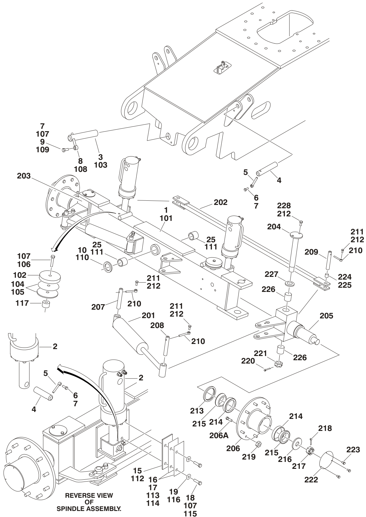
FIGURE 1-1. 2WD FRONT AXLE & STEERING INSTALLATIONS (S/N 0300069000 TO S/N 0300081836)
