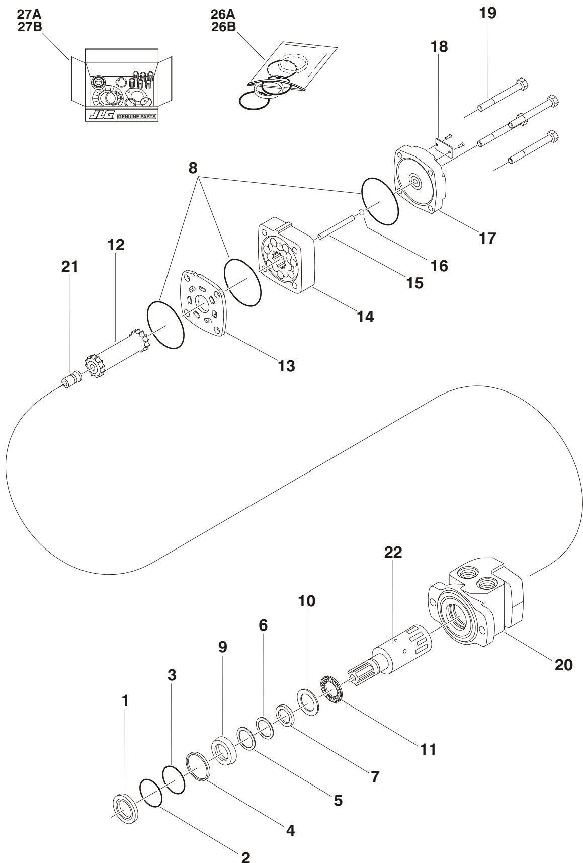
FIGURE 2-6. SWING MOTOR ASSEMBLY
