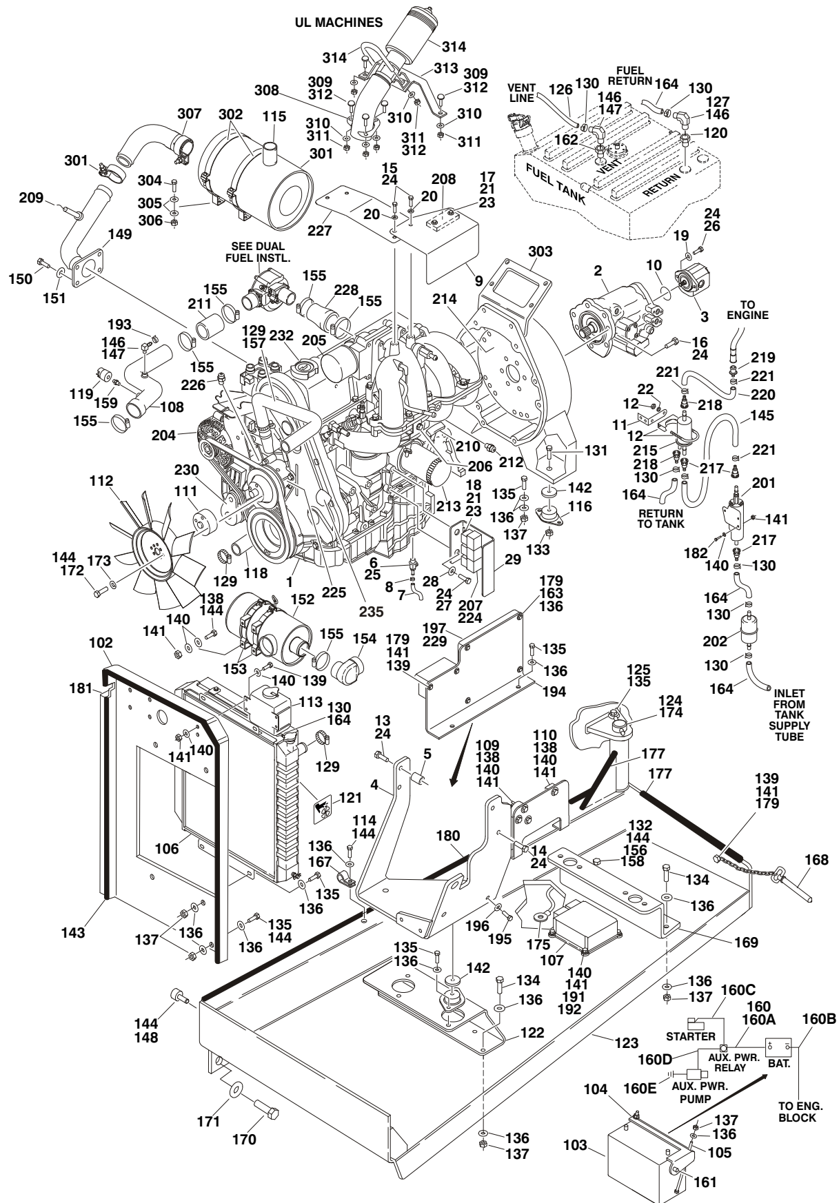
FIGURE 2-10. FORD ENGINE INSTALLATION - LRG-425 (S/N 0300069000 TO S/N 0300079888)
