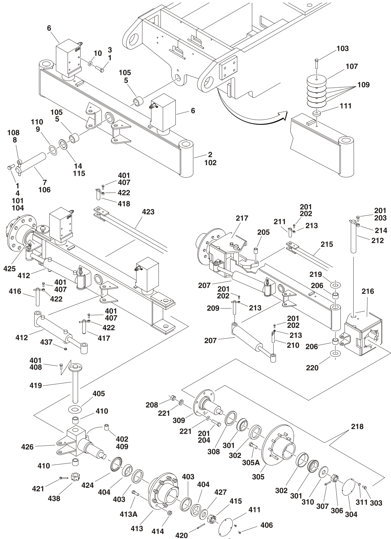
FIGURE 1-2. 2WD FRONT AXLE & STEERING INSTALLATIONS (S/N 0300081836 TO S/N 0300087000)
