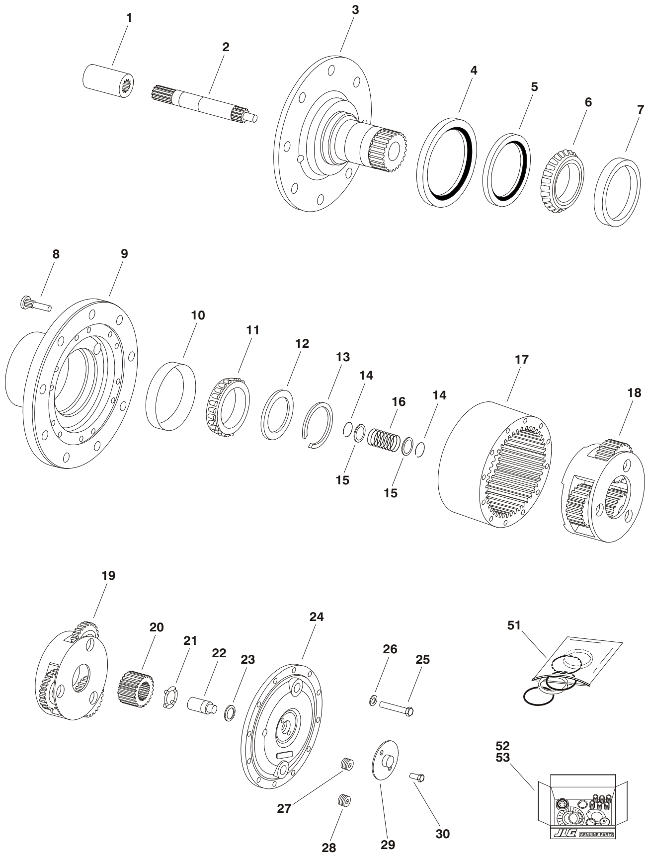
FIGURE 1-8. DRIVE HUB ASSEMBLY (S/N 0300069000 TO S/N 0300081836)
