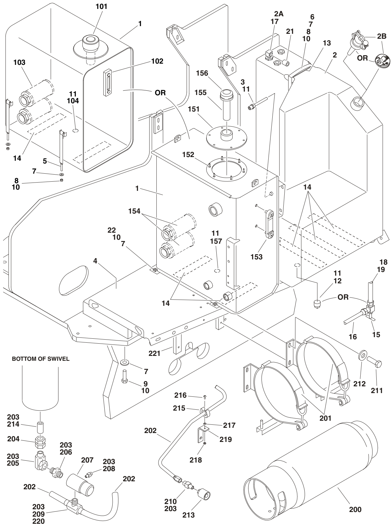
FIGURE 2-16. TANK INSTALLATIONS
