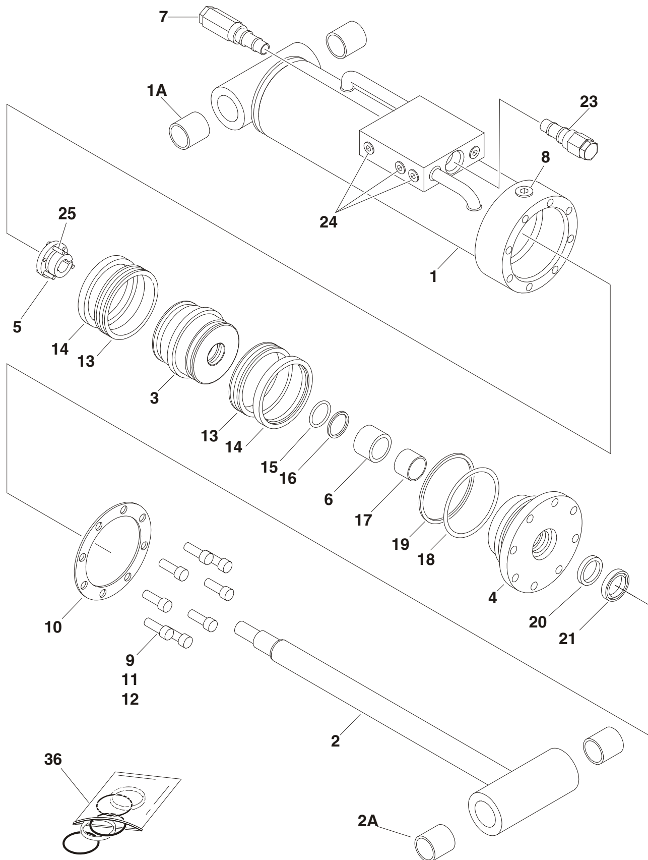
FIGURE 5-3. PLATFORM LEVEL CYLINDER ASSEMBLY
