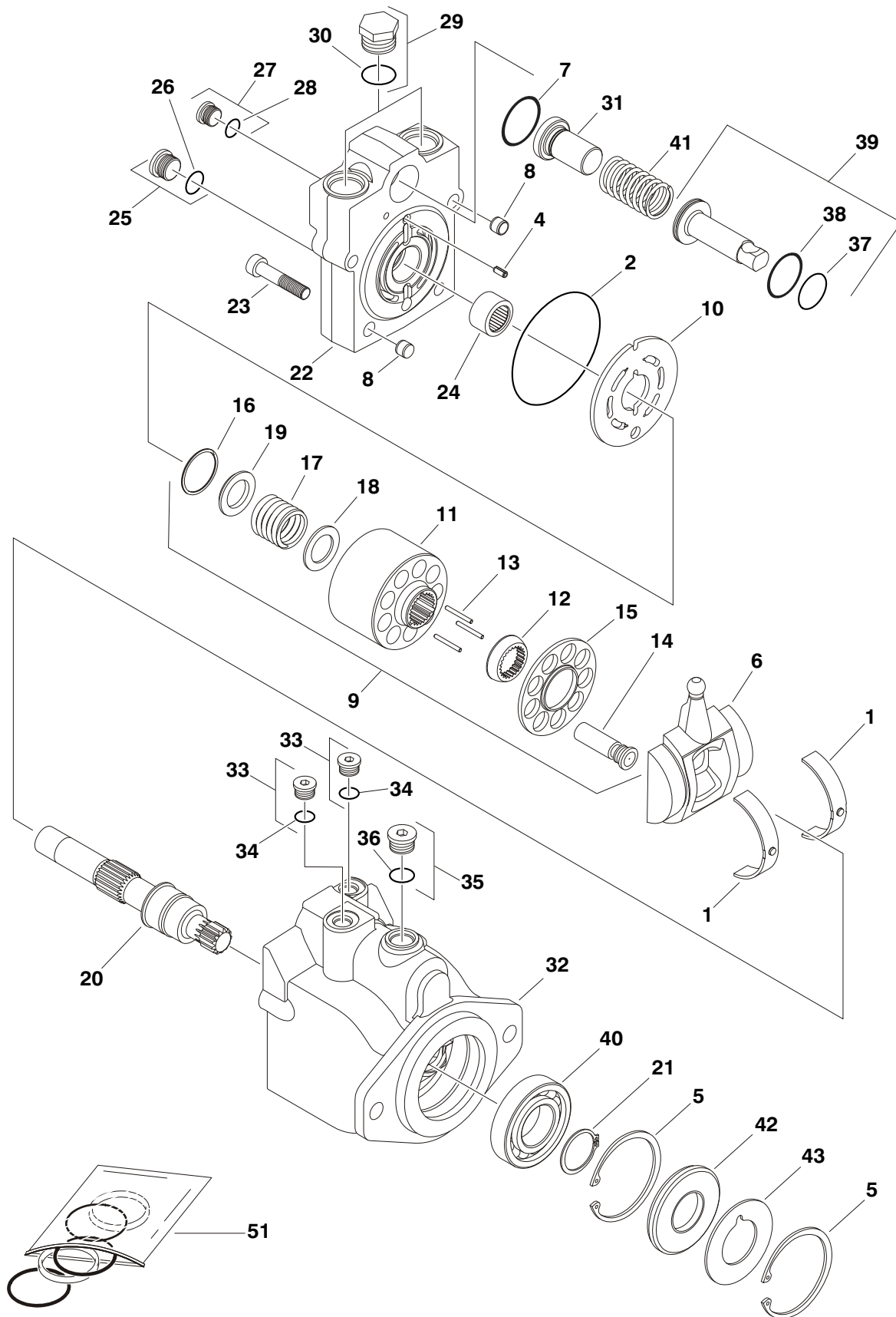
FIGURE 1-13. DRIVE MOTOR ASSEMBLY (2WD & 4WD MACHINES S/N 0300081836 TO S/N 0300087000) (ORIGINAL EQUIPMENT)
