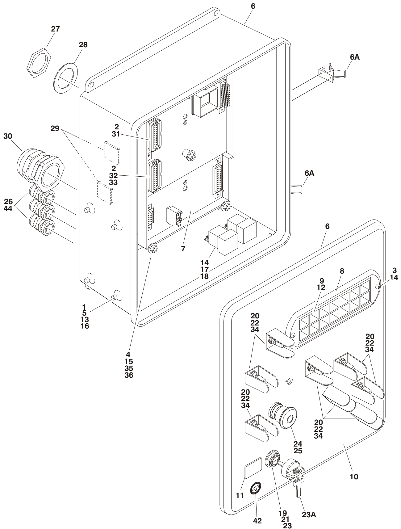
FIGURE 2-19. GROUND CONTROL BOX ASSEMBLIES
