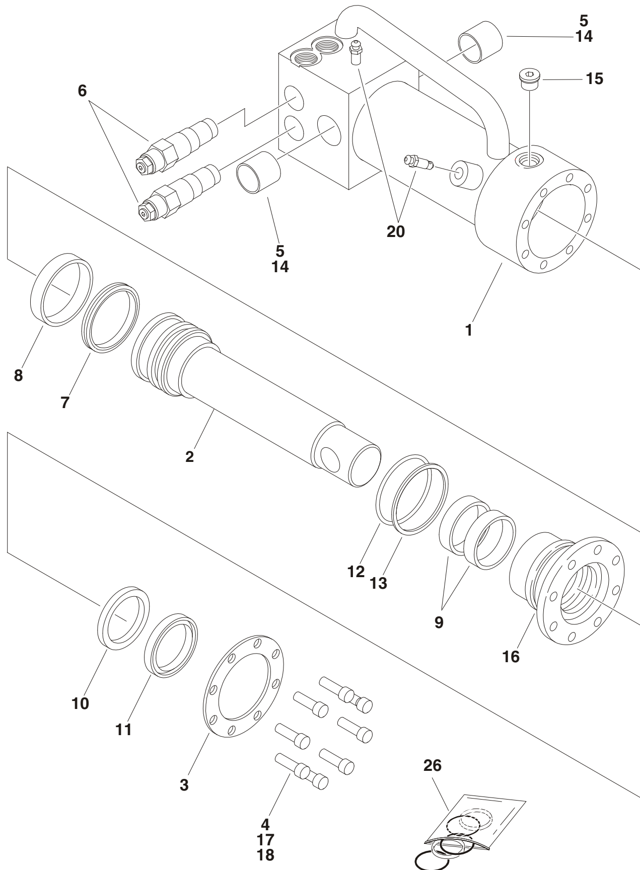
FIGURE 5-1. AXLE LOCKOUT CYLINDER ASSEMBLY (S/N 0300069000 TO S/N 0300081836)
