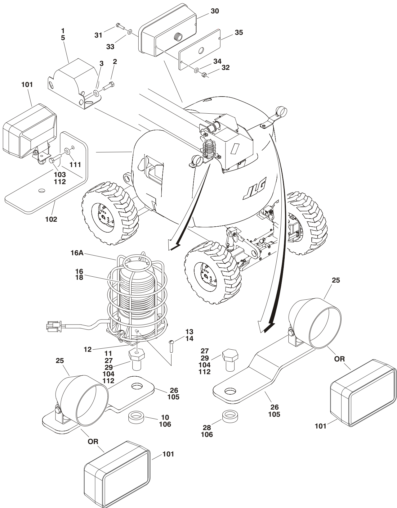
FIGURE 2-20. ELECTRICAL OPTIONS INSTALLATIONS (TURNTABLE MOUNTED)
