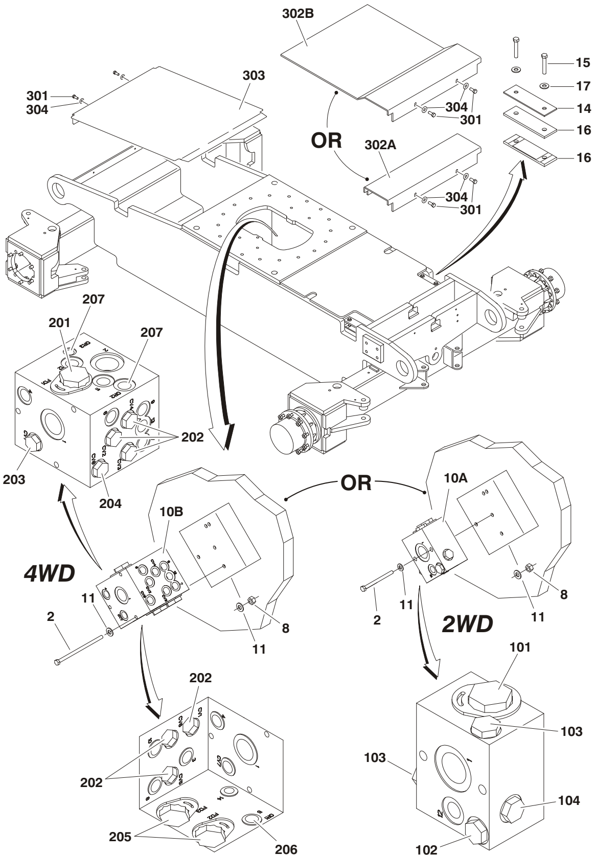
FIGURE 1-16. DRIVE VALVES & SHIELDS INSTALLATION (FRAME MOUNTED) (S/N 0300081836 TO S/N 0300087000)
