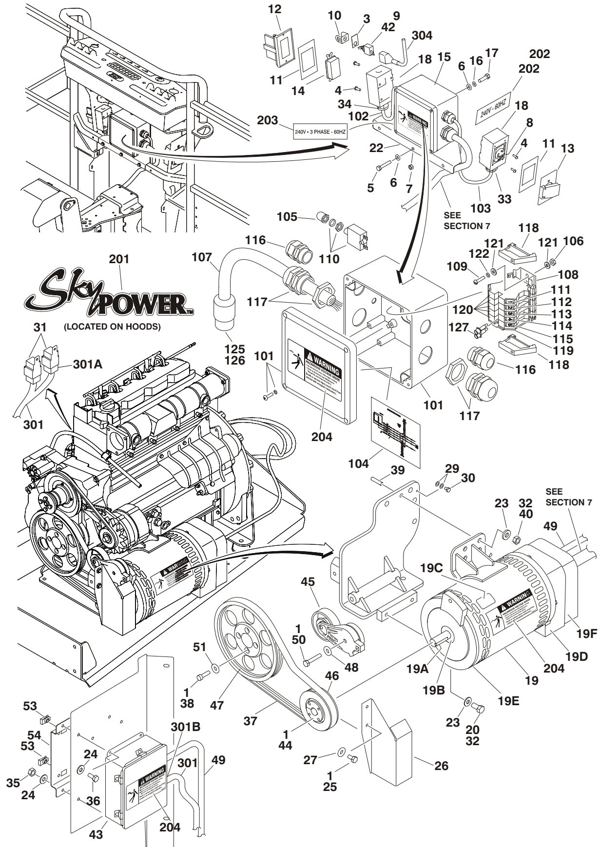
FIGURE 2-27. 7500W SKYPOWER GENERATOR INSTALLATION - CATERPILLAR & DEUTZ ENGINES
