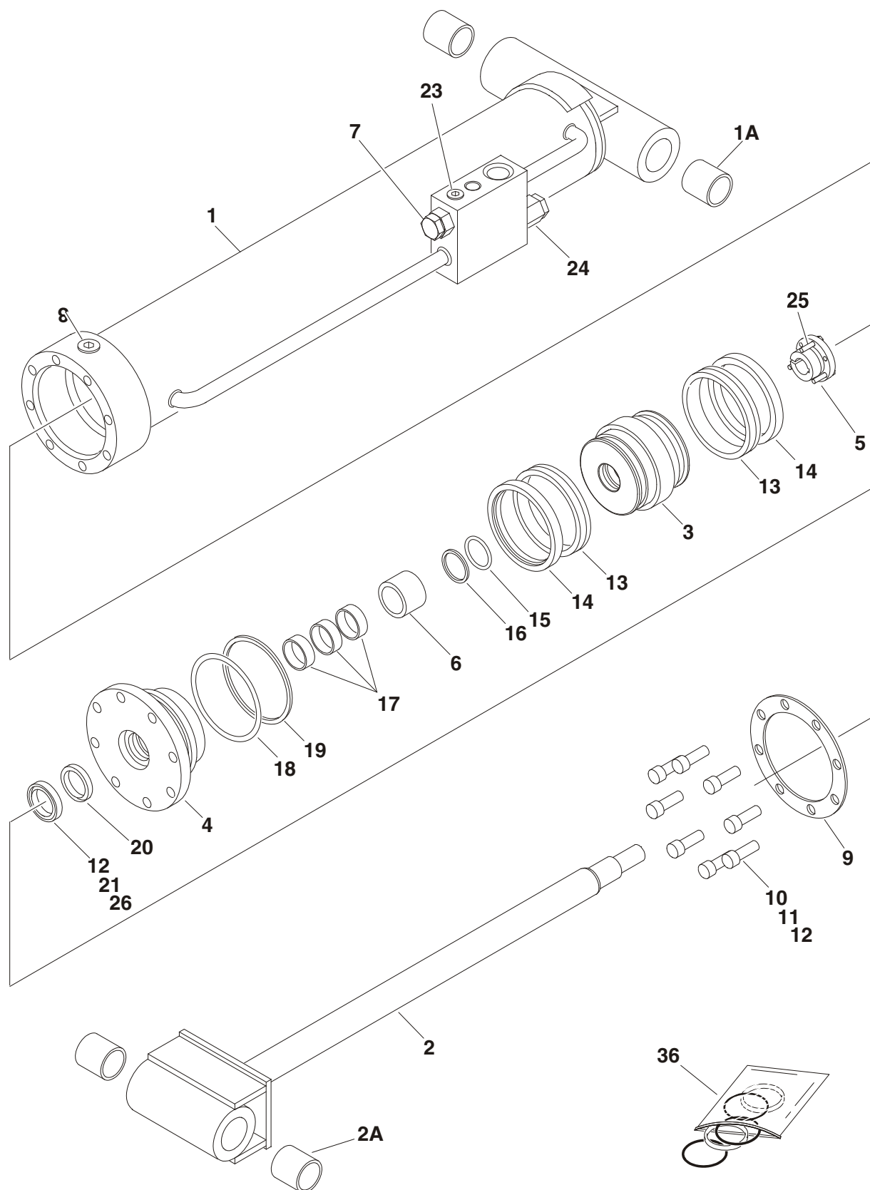
FIGURE 5-7. LIFT CYLINDER ASSEMBLY - TOWER BOOM
