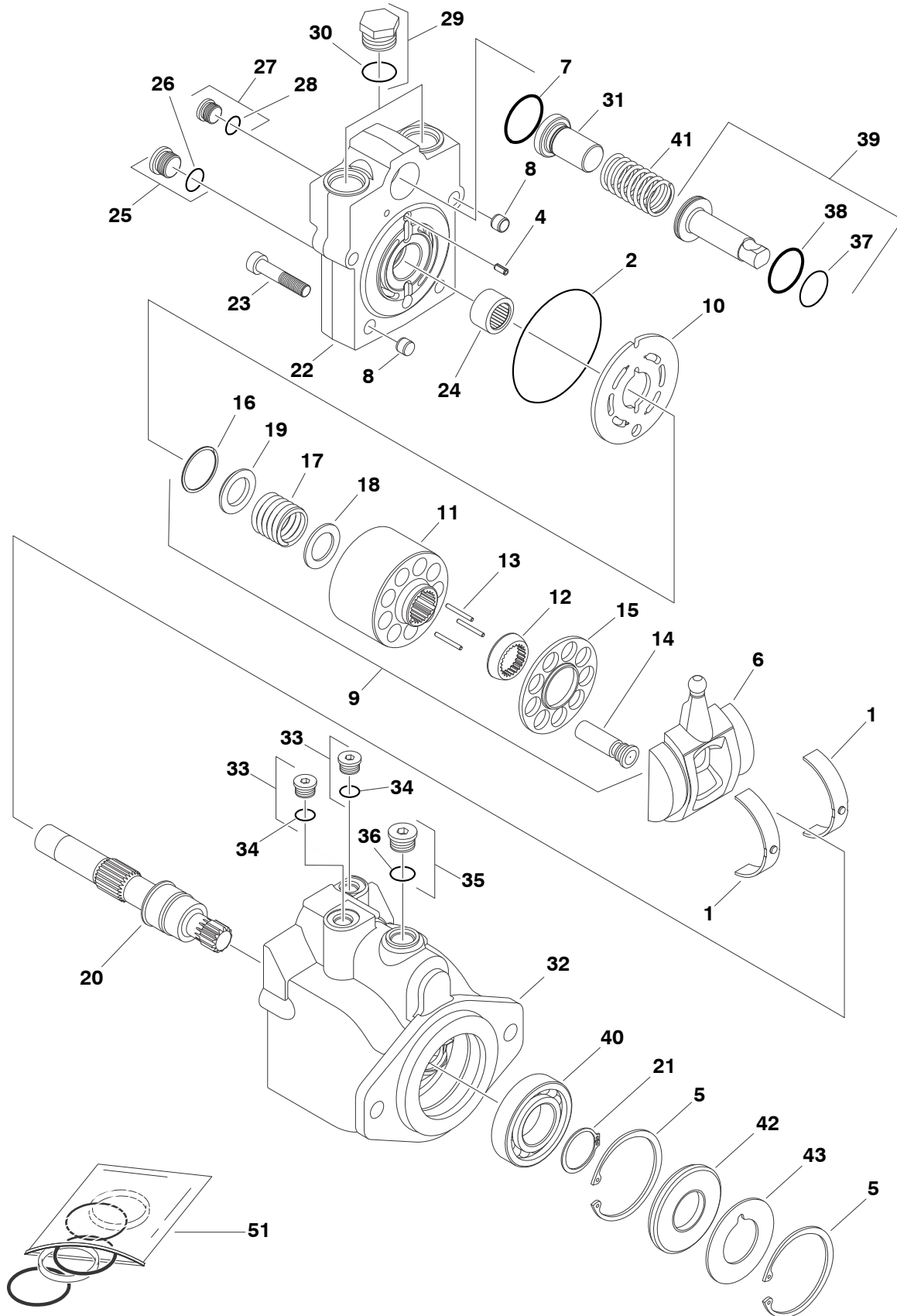
FIGURE 1-14. DRIVE MOTOR ASSEMBLY (2WD & 4WD MACHINES) (SERVICE REPLACEMENT)
