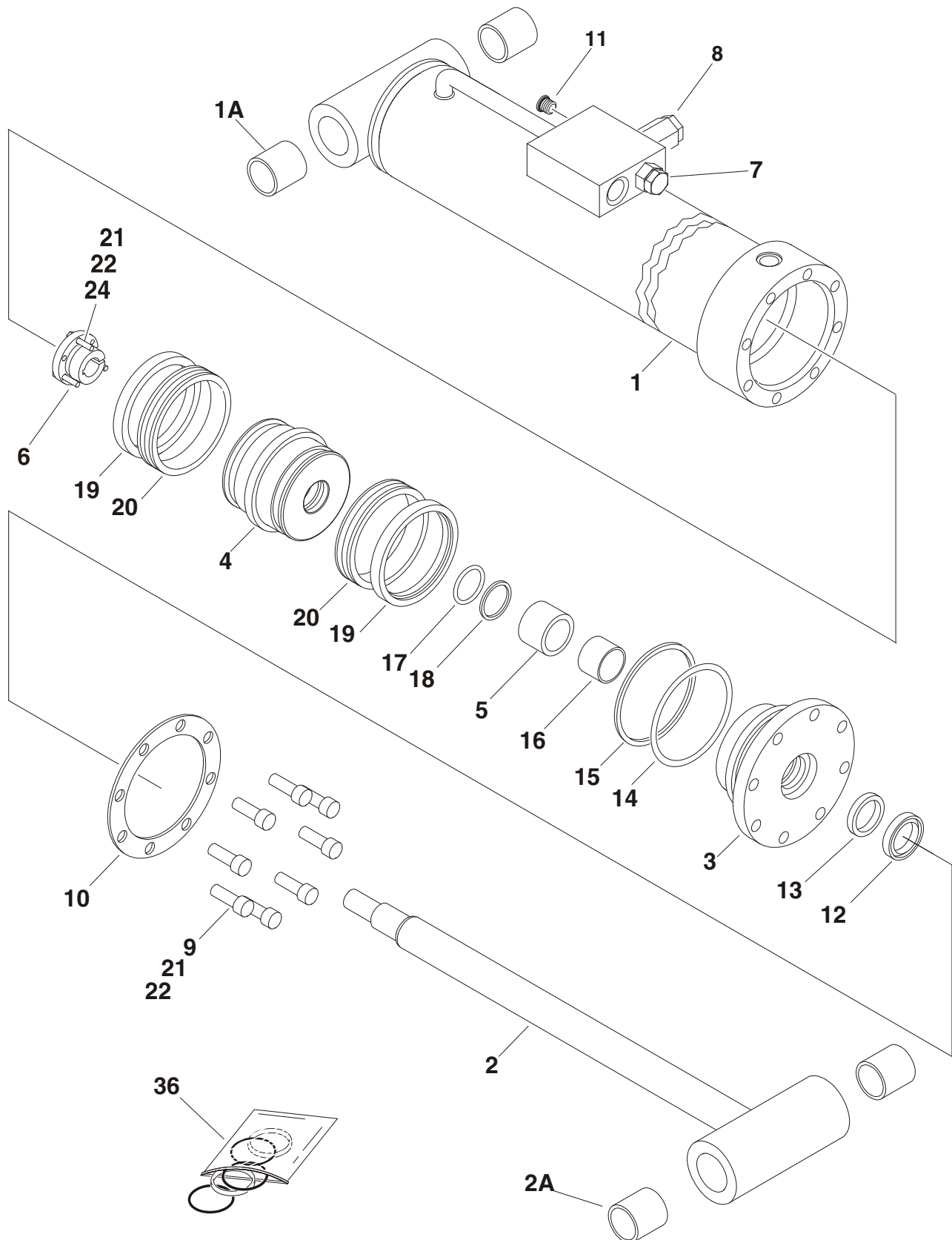
FIGURE 5-6. LIFT CYLINDER ASSEMBLY - MAIN BOOM
