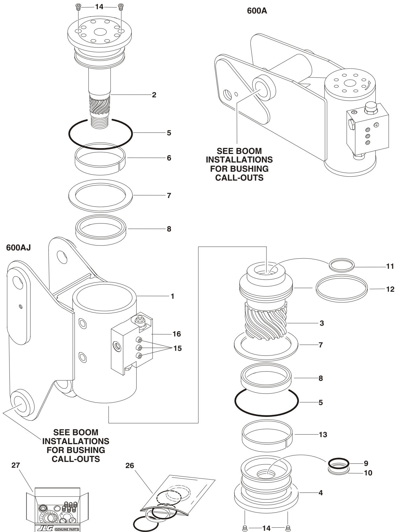
FIGURE 3-6. ROTATOR ASSEMBLIES (SIDE ENTRY PLATFORM)
