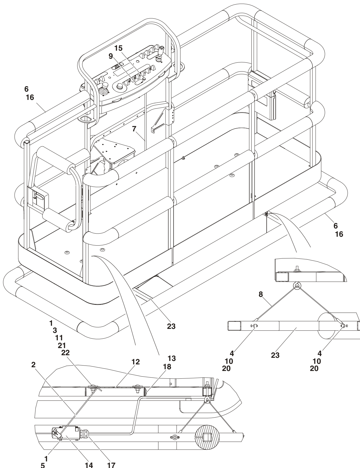
FIGURE 4-7. SOFT TOUCH SYSTEM INSTALLATION (OPTIONAL)
