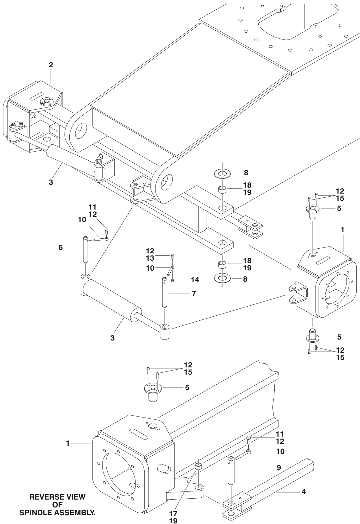
FIGURE 1-5. 4WS REAR STEERING INSTALLATIONS (S/N 0300069000 TO S/N 0300081836)
