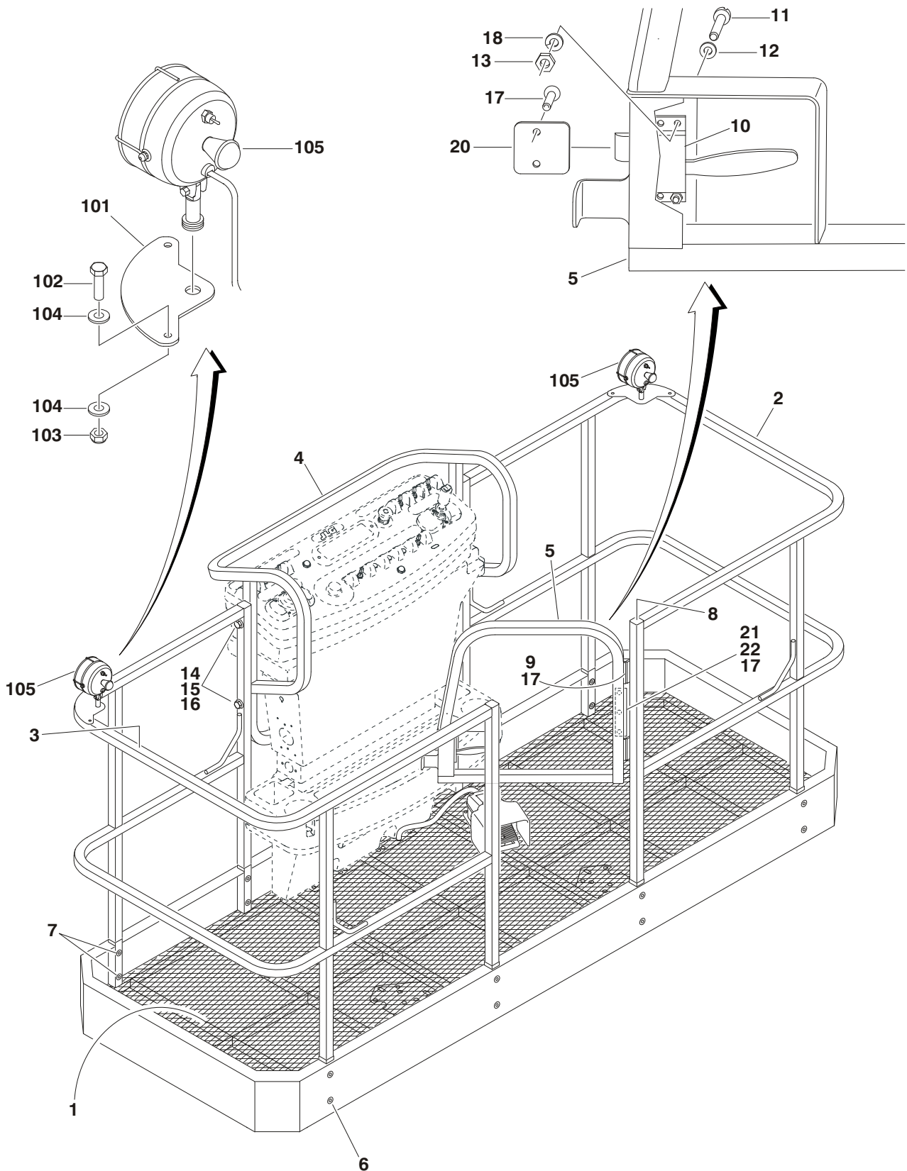
FIGURE 4-1. PLATFORM ASSEMBLIES (FRONT ENTRY PLATFORM)
