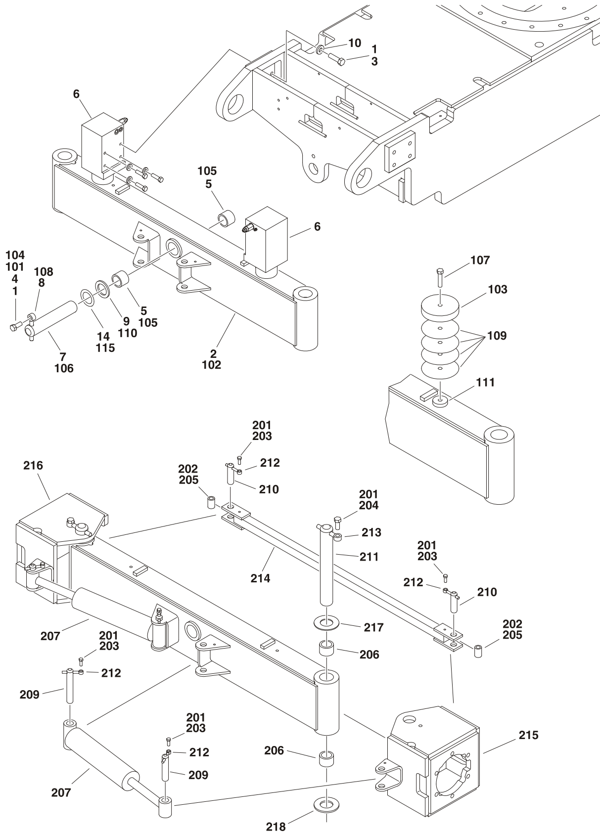
FIGURE 1-4. 4WD FRONT AXLE & STEERING INSTALLATIONS (S/N 0300081836 TO S/N 0300087000)
