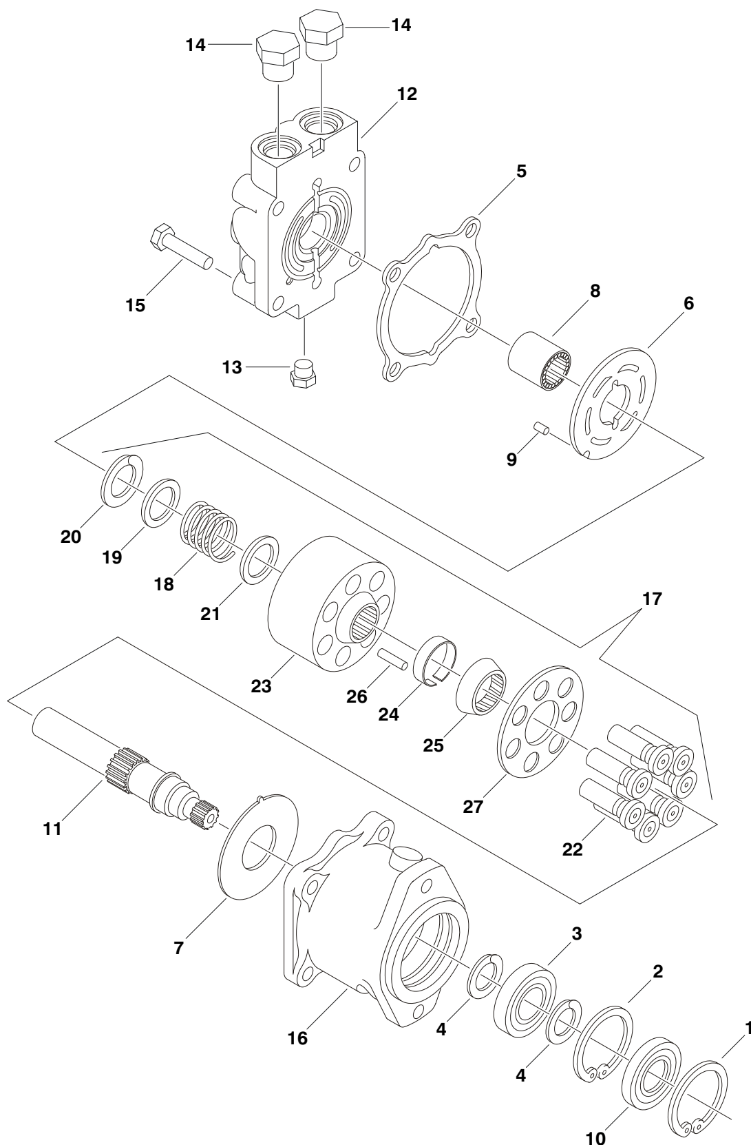
FIGURE 1-10. DRIVE MOTOR ASSEMBLY (2WD MACHINES S/N 0300069000 TO S/N 0300071020)
