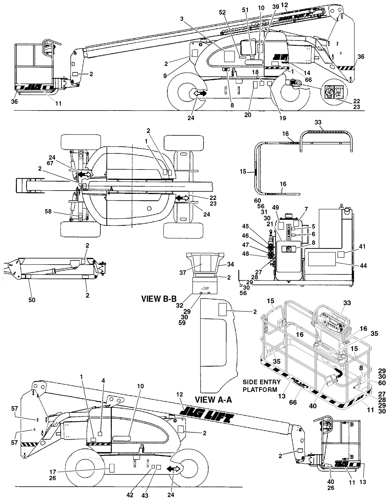
FIGURE 8-3. DECAL INSTALLATION (COUNTRY SPECS) (S/N 0300069000 TO S/N 0300086150)
