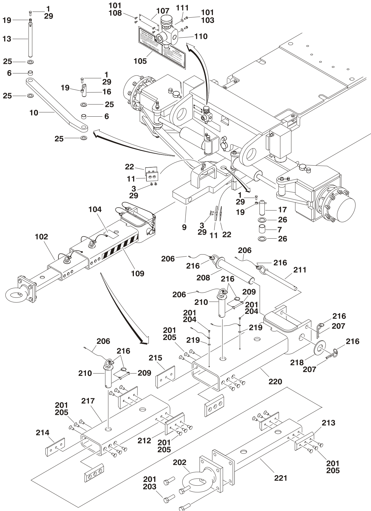
FIGURE 1-18. TOW PACKAGE INSTALLATION (S/N 0300081836 TO S/N 0300087000) (OPTIONAL)
