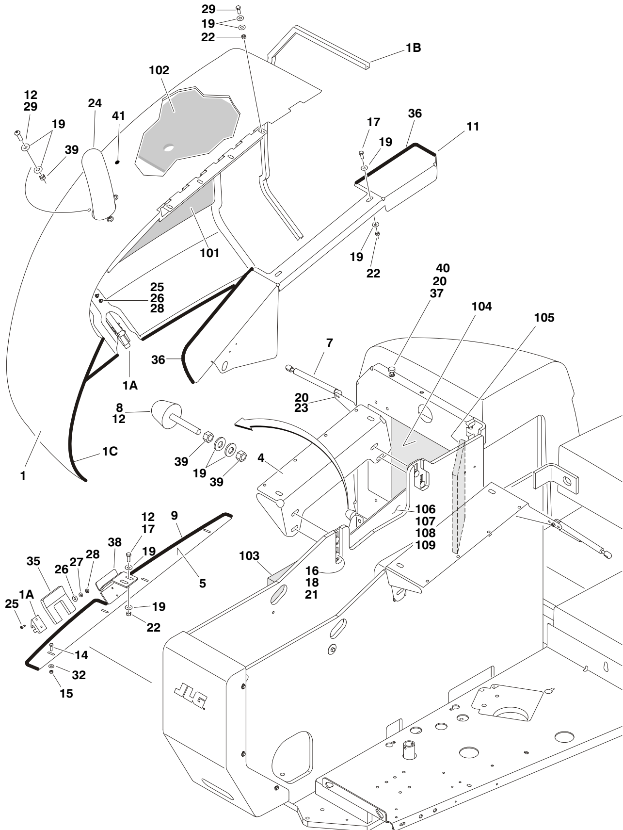
FIGURE 2-22. HOODS INSTALLATIONS
