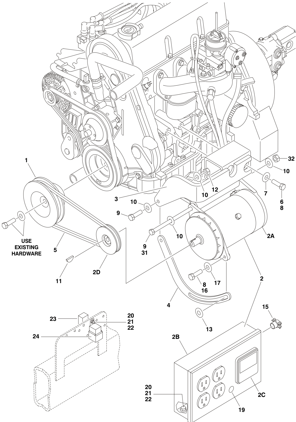
FIGURE 2-25. 2500W GENERATOR INSTALLATION - FORD MACHINES (OPTIONAL) (S/N 0300069000 TO S/N 0300079888)
