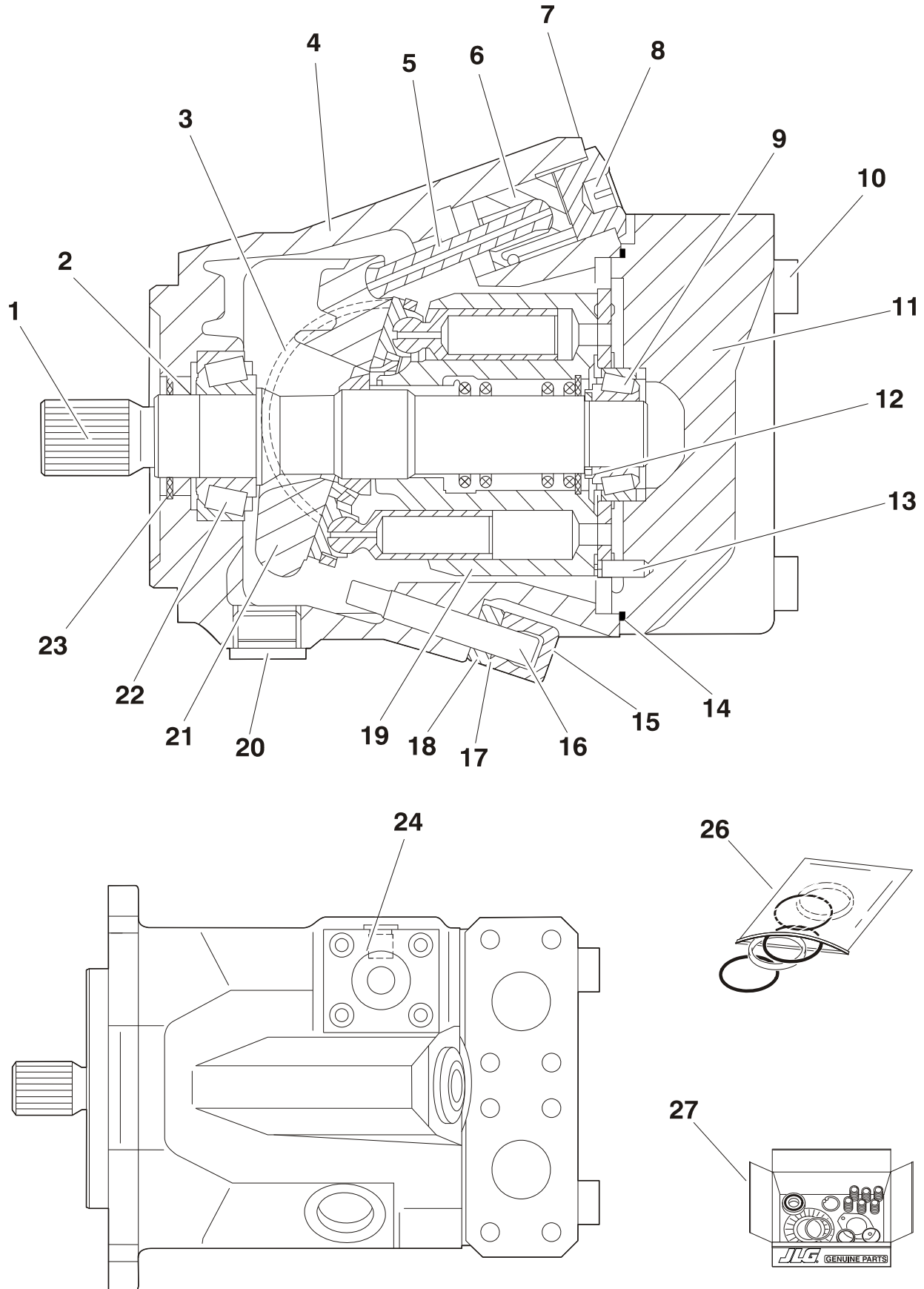
FIGURE 1-12. DRIVE MOTOR ASSEMBLY (4WD MACHINES S/N 0300069000 TO S/N 0300081836)
