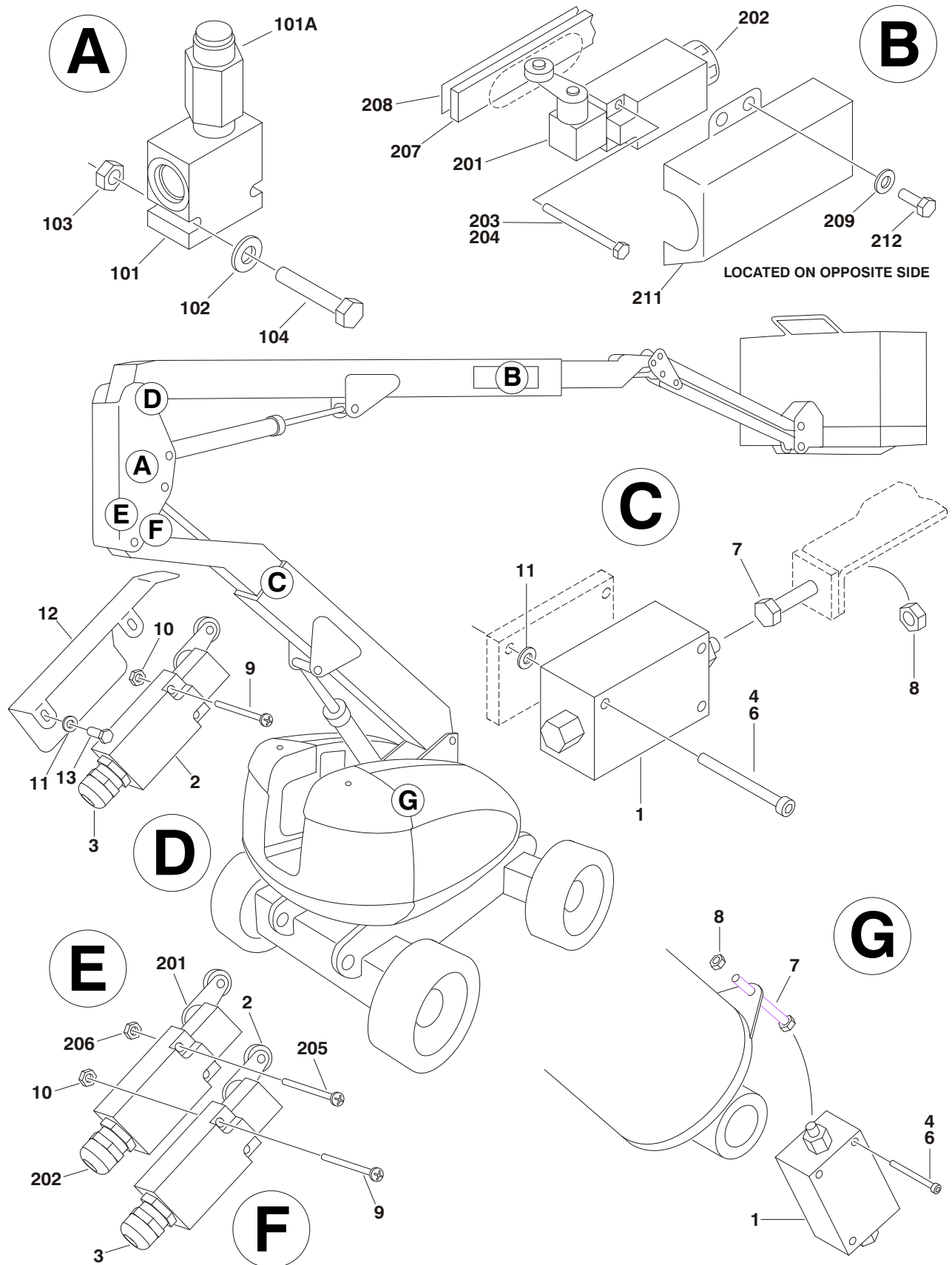
FIGURE 3-7. VALVES & SWITCHES INSTALLATION (BOOM MOUNTED)
