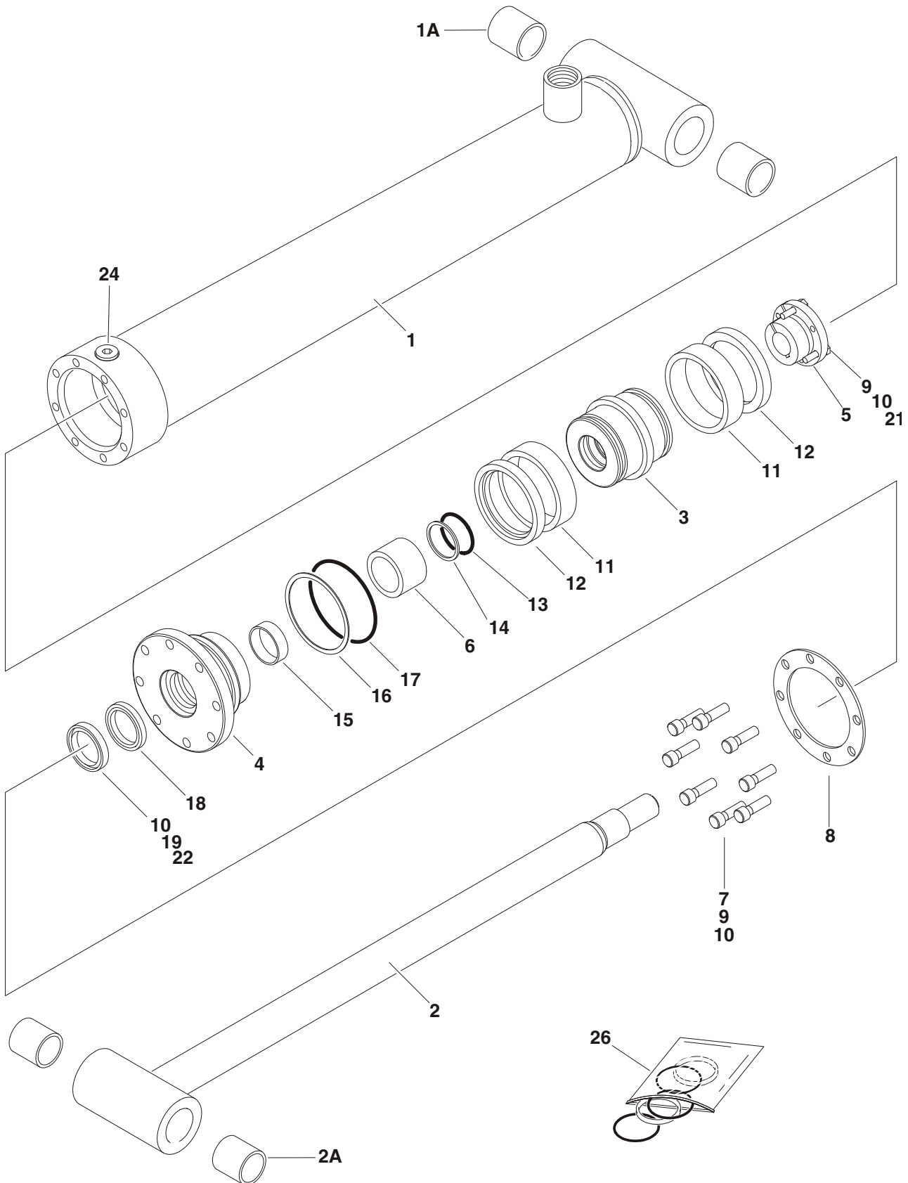
FIGURE 5-8. MASTER CYLINDER ASSEMBLY
