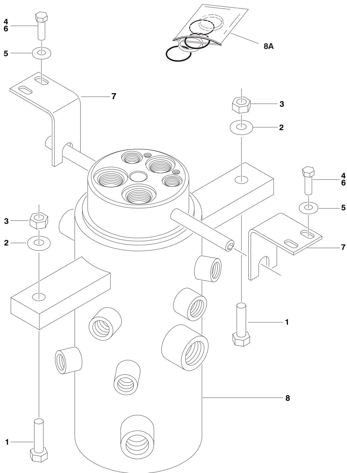
FIGURE 2-17. ROTARY COUPLING INSTALLATIONS (S/N 0300069000 TO S/N 0300081836)
