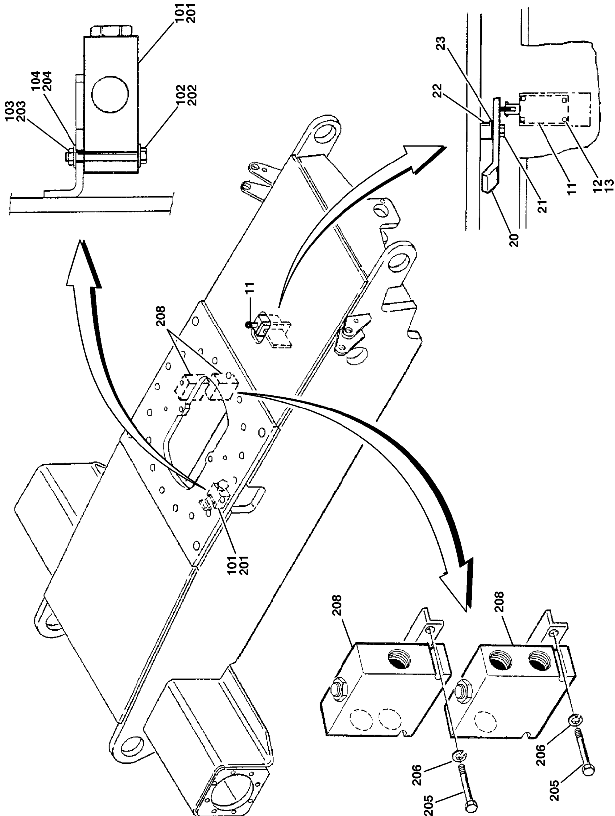
FIGURE 1-15. DRIVE VALVES & SHIELDS INSTALLATION (FRAME MOUNTED) (S/N 0300069000 TO S/N 0300081836)
