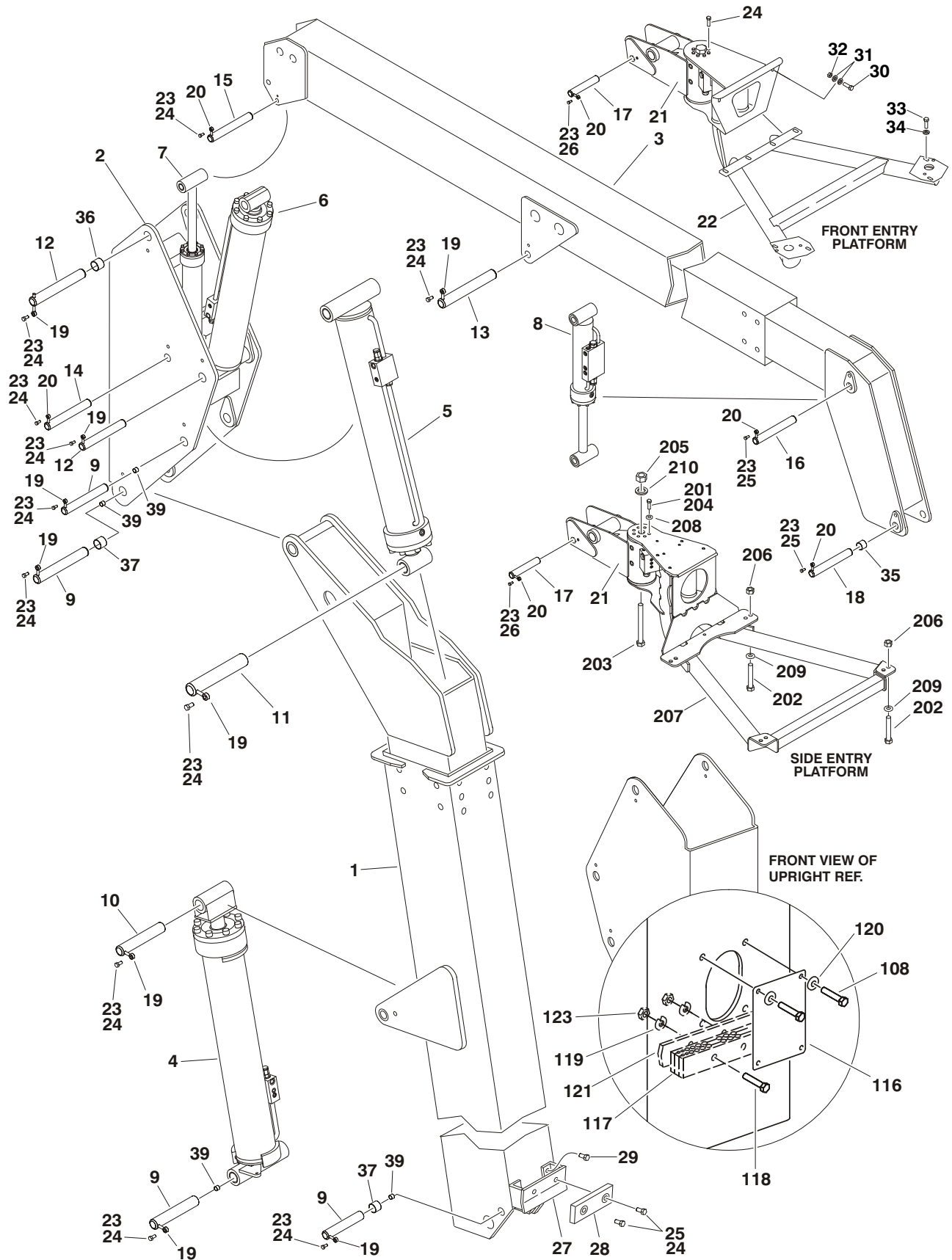
FIGURE 3-1. BOOMS & CYLINDERS INSTALLATION - 600A
