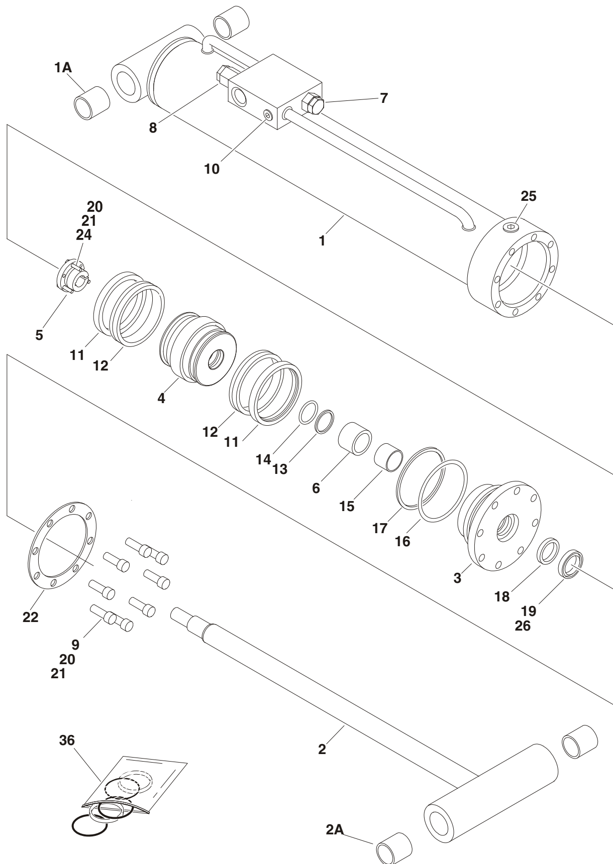
FIGURE 5-4. LEVEL CYLINDER ASSEMBLY - UPRIGHT
