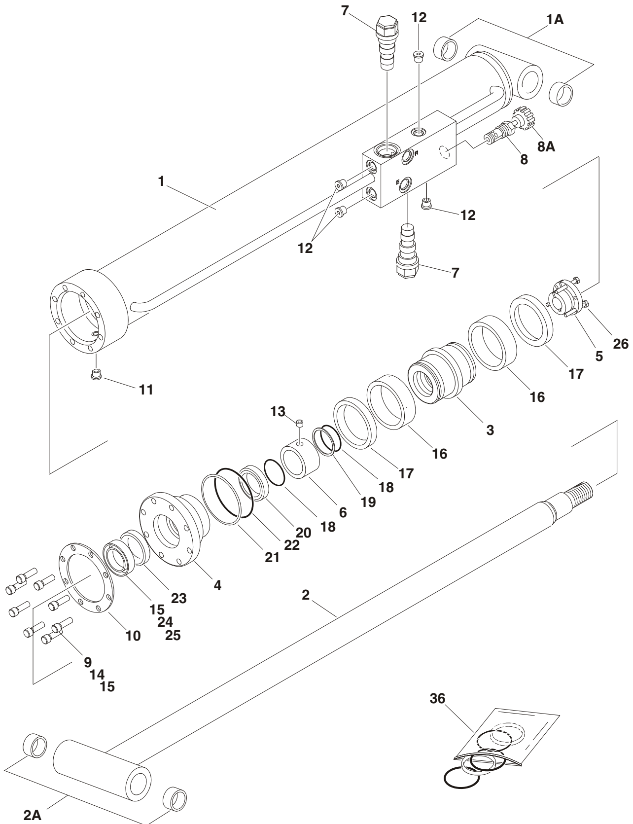
FIGURE 5-5. LIFT CYLINDER ASSEMBLY - ARTICULATING JIB
