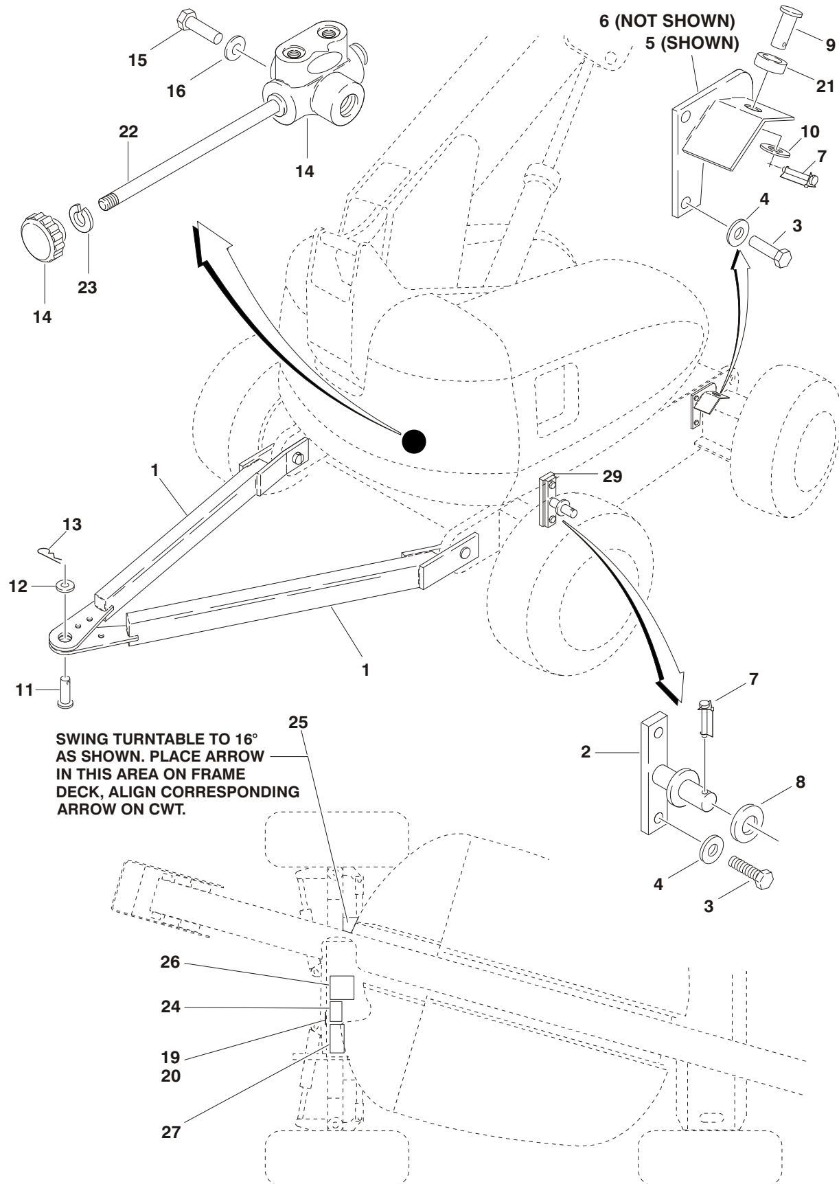
FIGURE 1-17. TOW PACKAGE INSTALLATION (S/N 0300069000 TO S/N 0300081836) (OPTIONAL)
