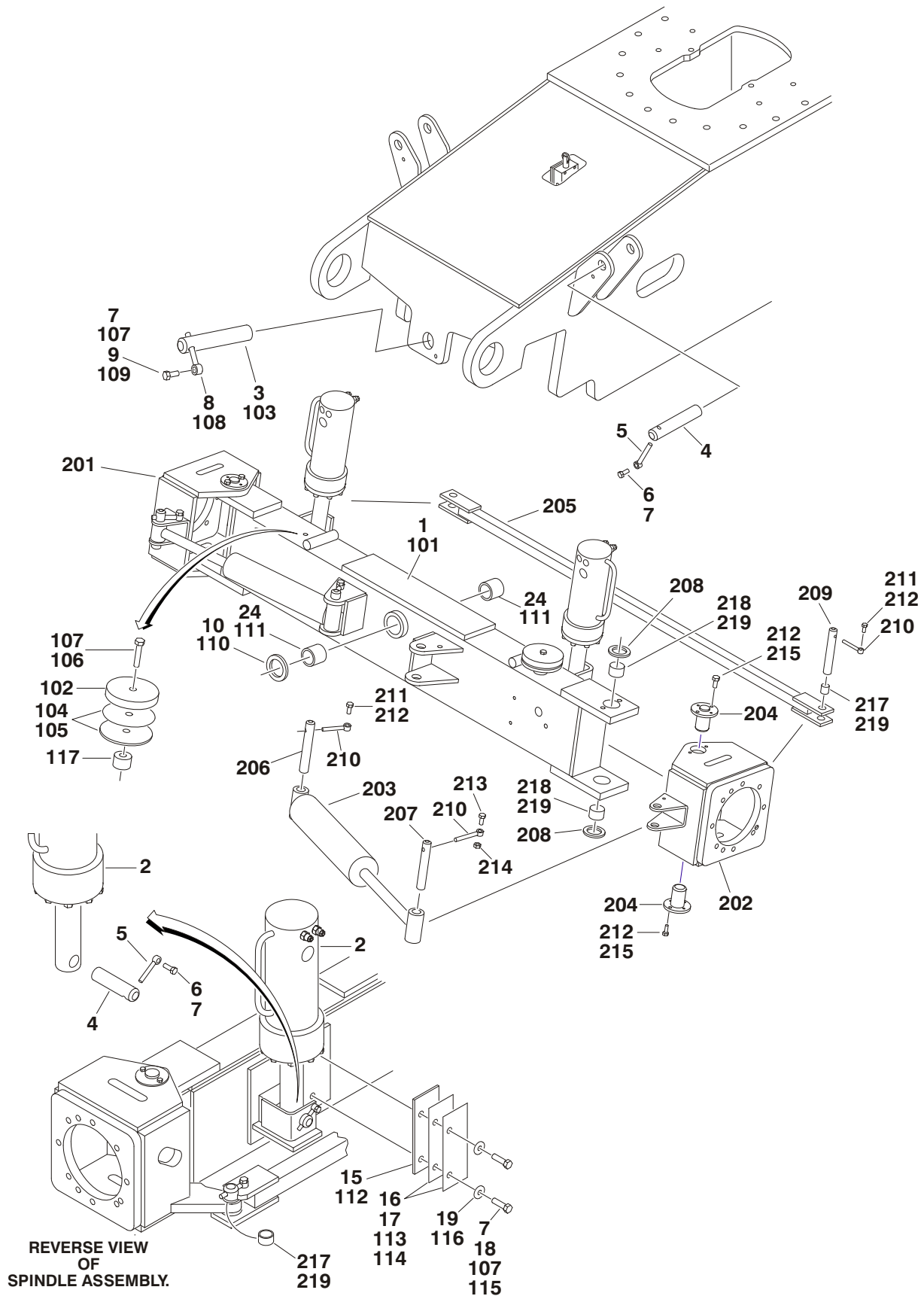
FIGURE 1-3. 4WD FRONT AXLE & STEERING INSTALLATIONS (S/N 0300069000 TO S/N 0300081836)
