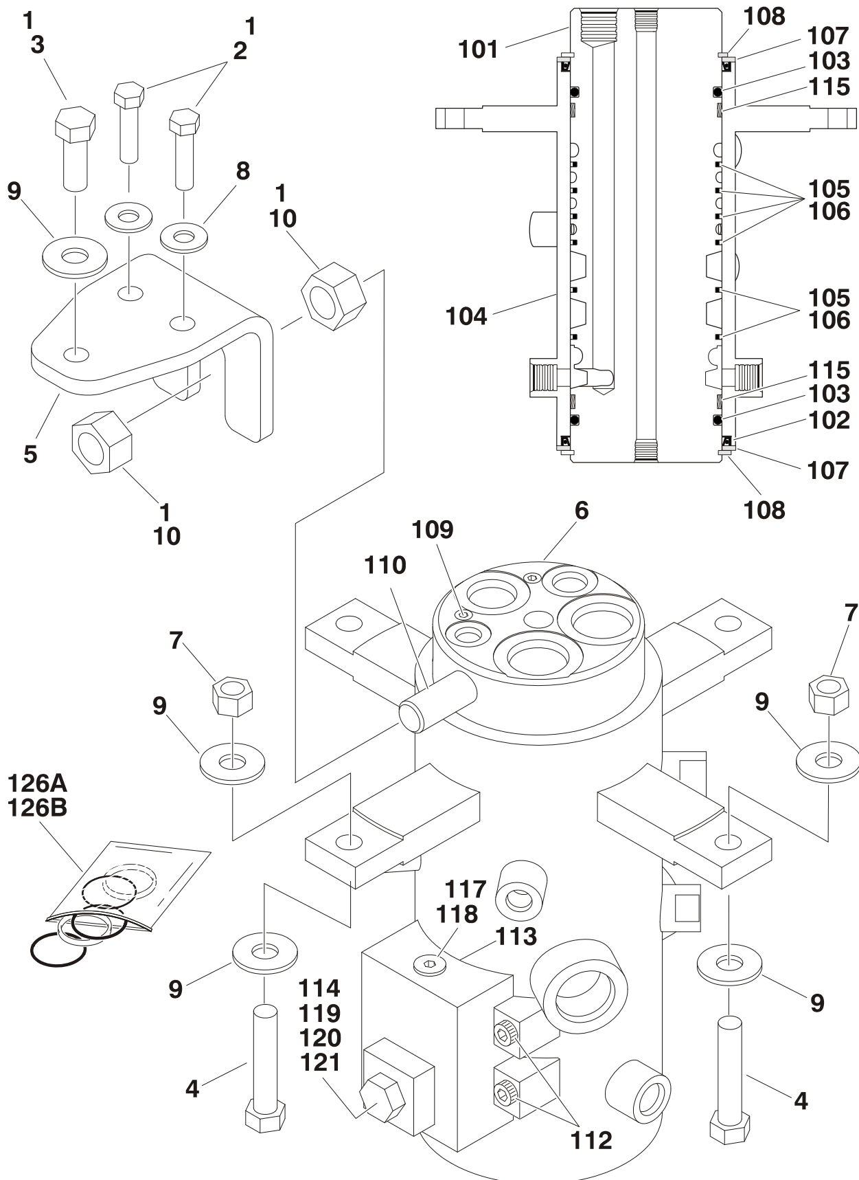
FIGURE 2-18. ROTARY COUPLING INSTALLATIONS (S/N 0300081836 TO S/N 0300087000)
