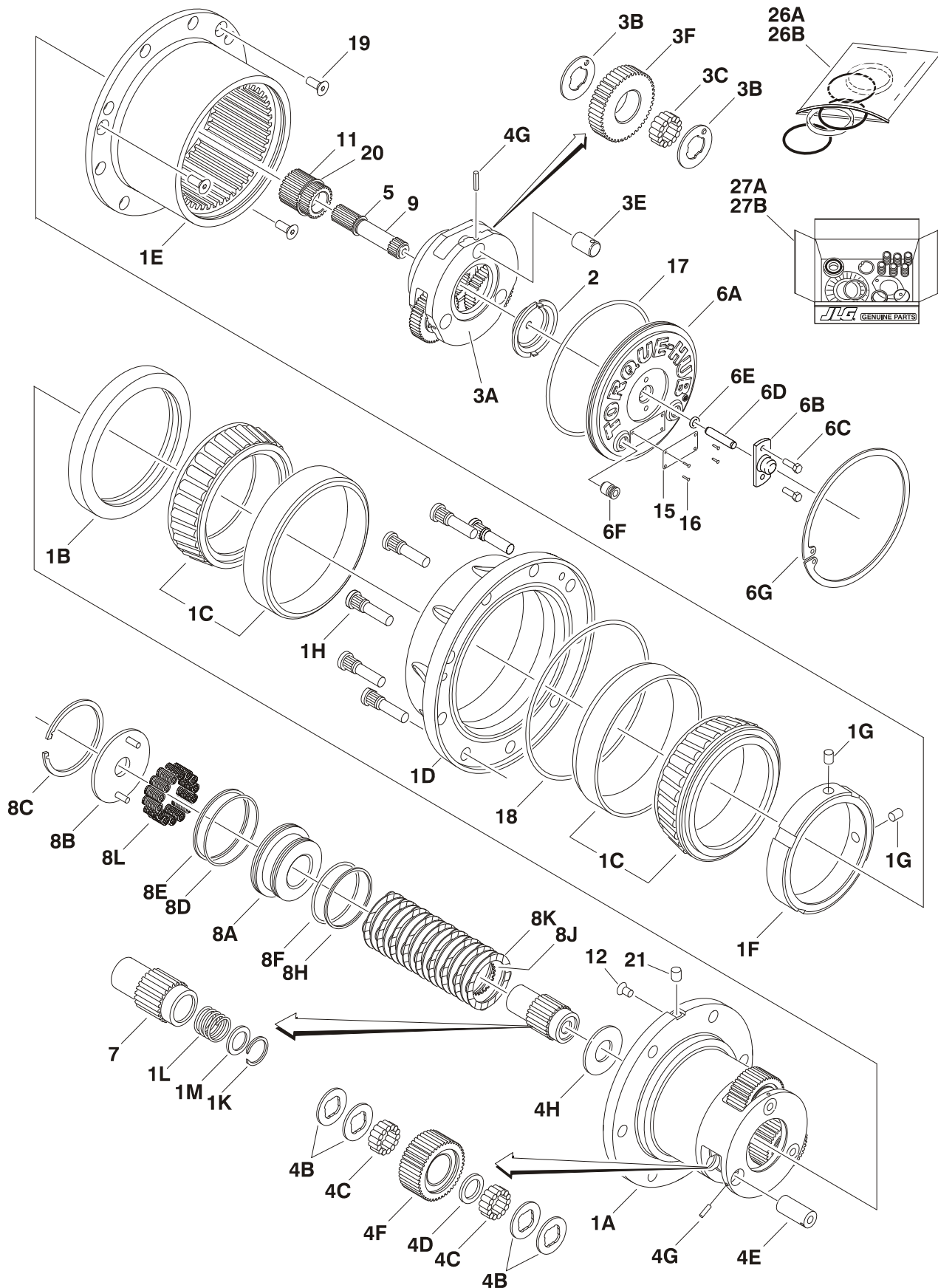
FIGURE 1-9. DRIVE HUB ASSEMBLY (S/N 0300081836 TO S/N 0300087000)
