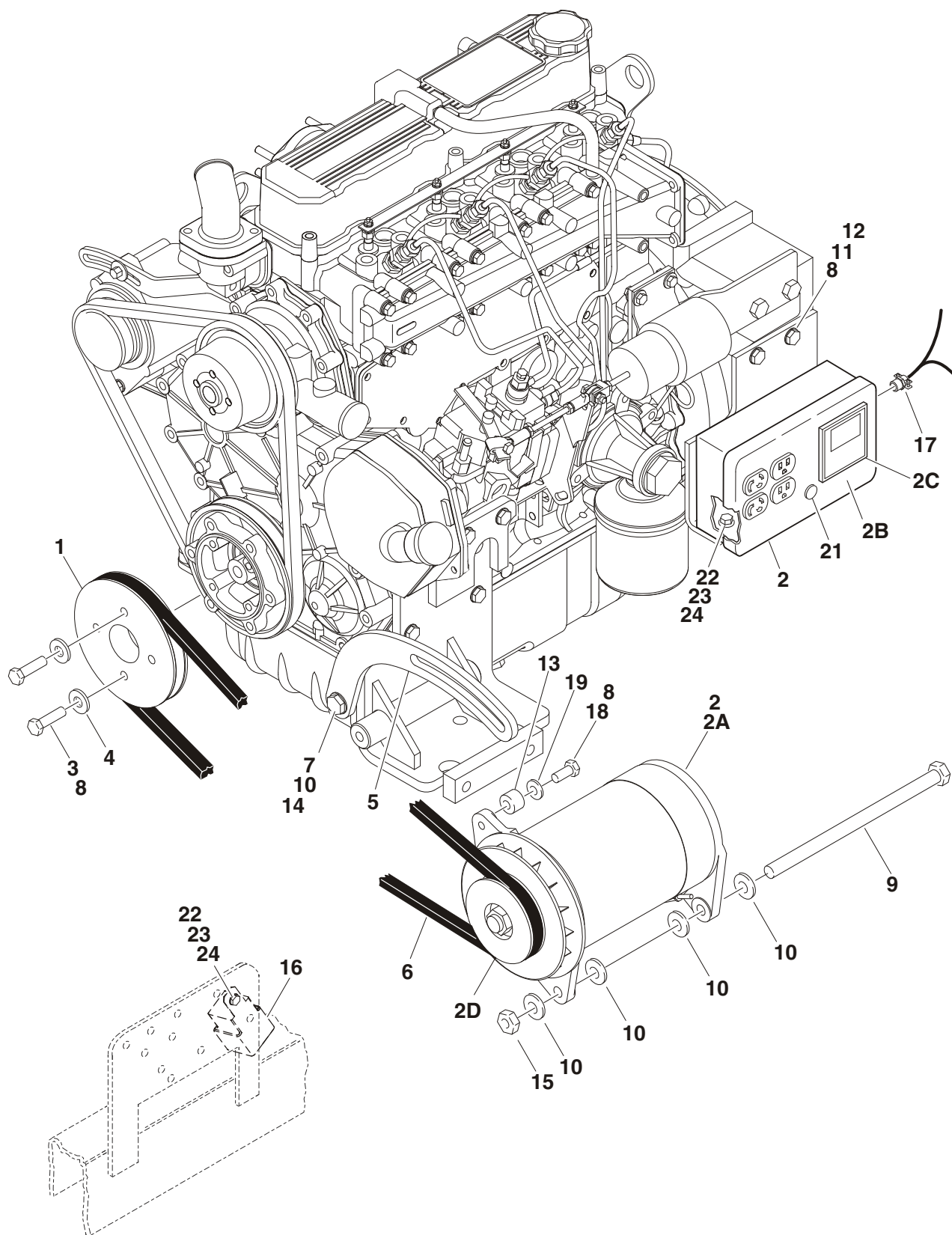
FIGURE 2-23. 2500W GENERATOR INSTALLATION - CATERPILLAR MACHINES (OPTIONAL)
